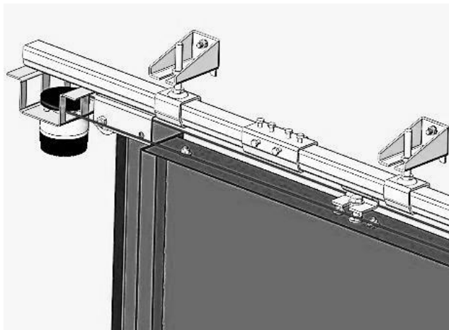
Brake and reverse pulley with wire rope under tension
