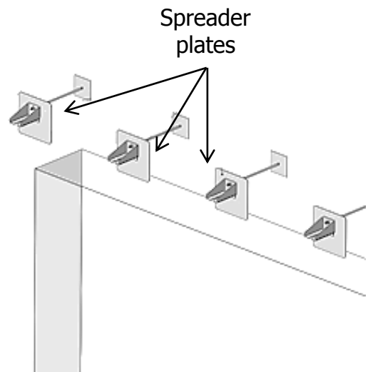
Anchoring by means of bolts through the wall
