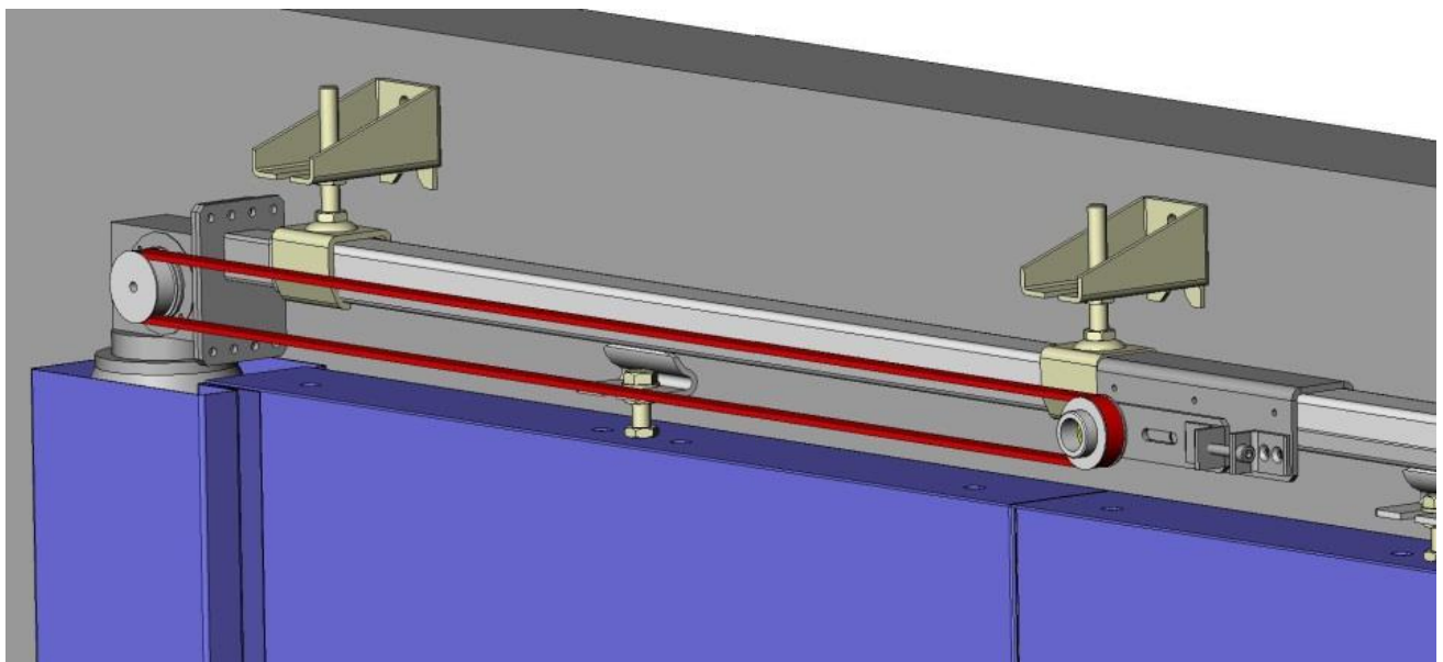
Motor bracket and reverse pulley with tightener
