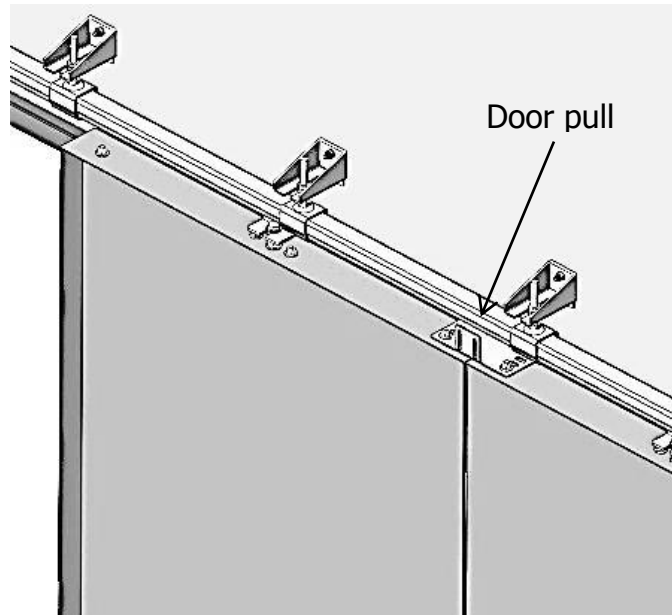
Placement of door pull
