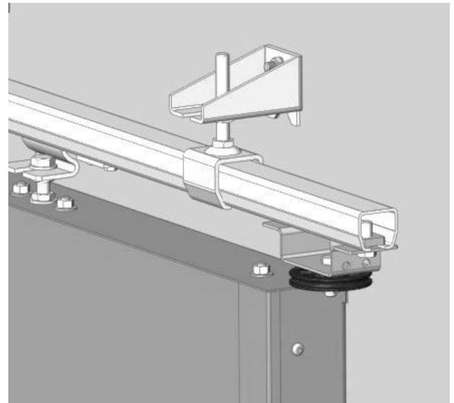
Placement of the reverse pulley
