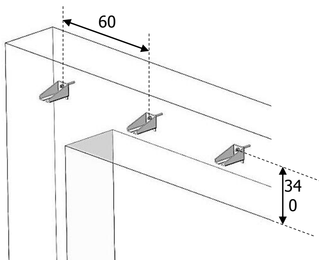
Anchoring by means of concrete anchors
