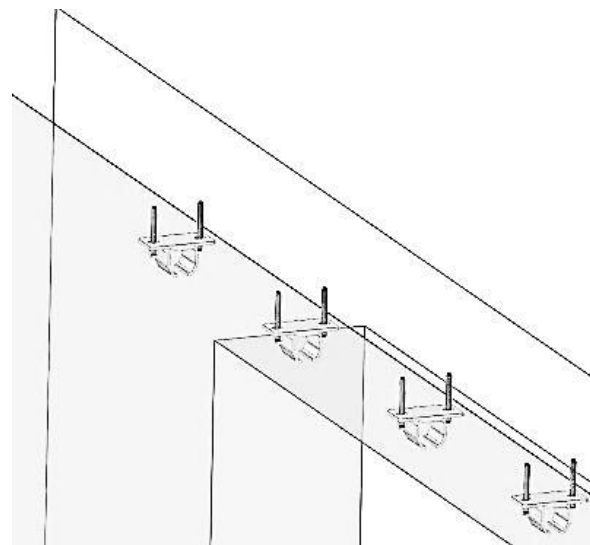
Anchoring to ceiling by means of concrete anchors
