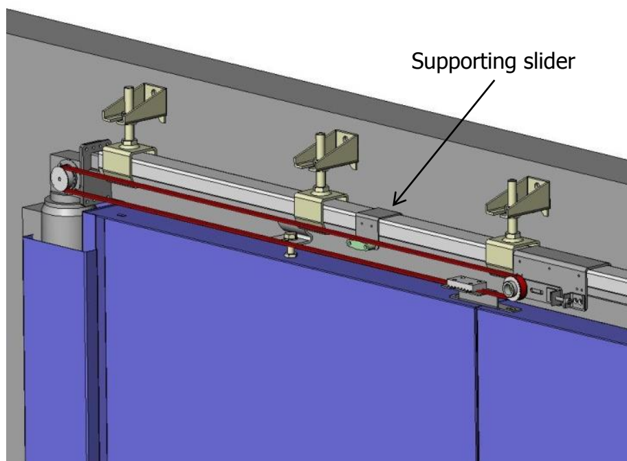
Belt with supporting slider
