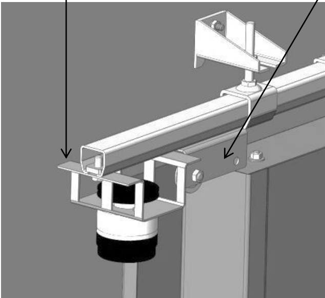
Placement of electromagnetic brake and bracket for the counterweight pulley
