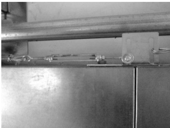
Door pull with screw turnbuckle
