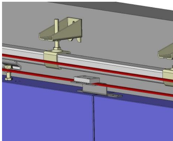
Door pull with clamping plate
